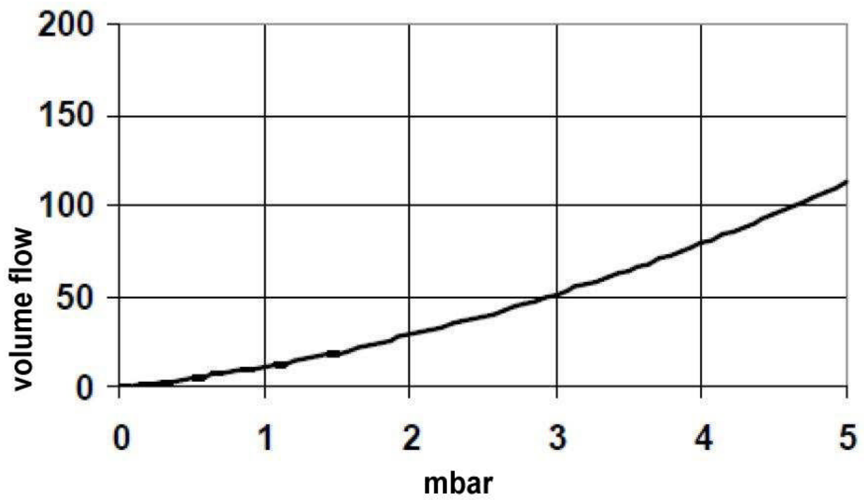
Pressure Drop chart BLUh - BLUhx
