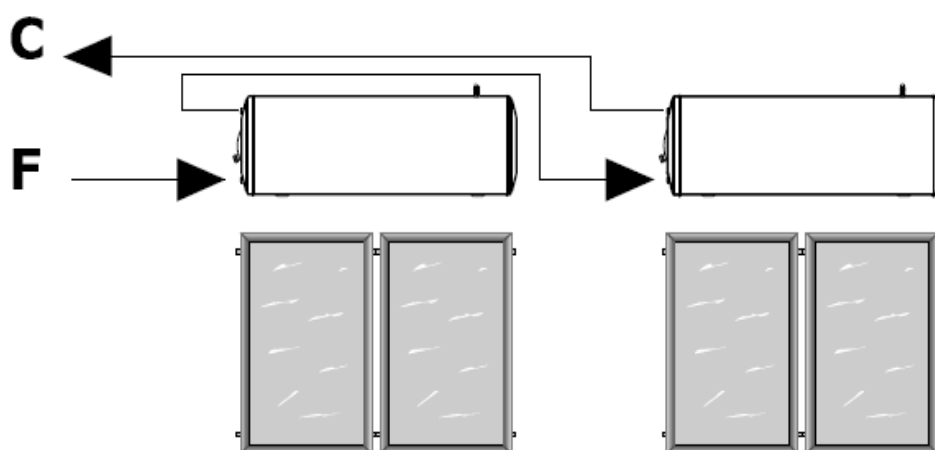
Collegamento in Serie Series connection
